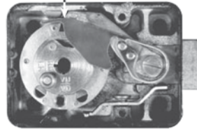
Accelerator Spring in Released Position
