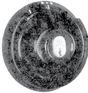
D112 with R162 3.753" (95.3mm) ring diameter B&W finish Four pin tumbler key lock: Function 3 only - non key retaining (National D4291 blank) This is the only Group 2 type dial with a pressed and pinned spindle.
