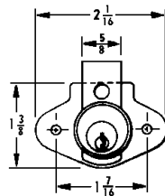
Key Blank: D4291
